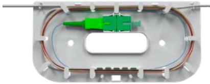
Internal view of Standard POE Module
